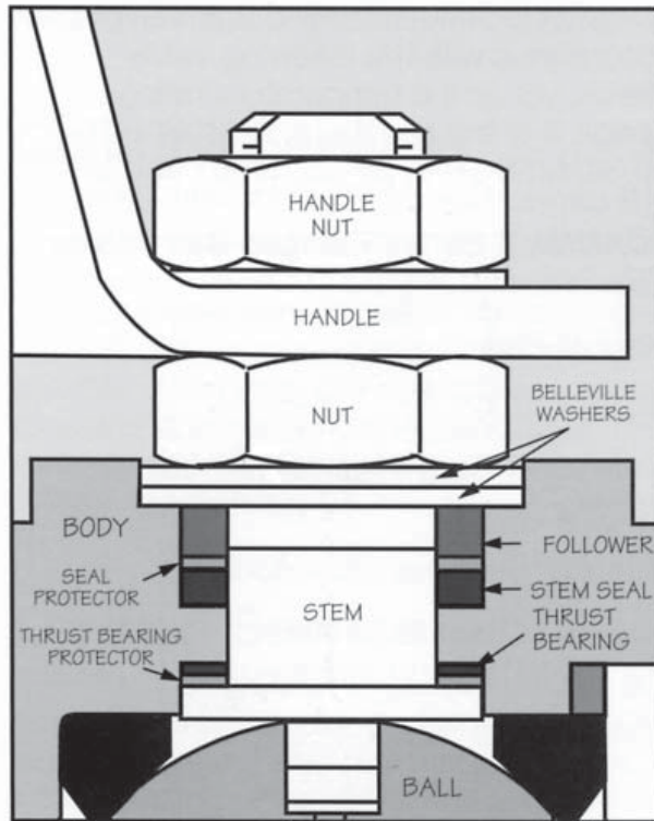
(Sizes 1/2" through 1 1/2" Regular Port)
