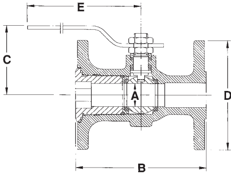
Sizes ½" – 1½"
