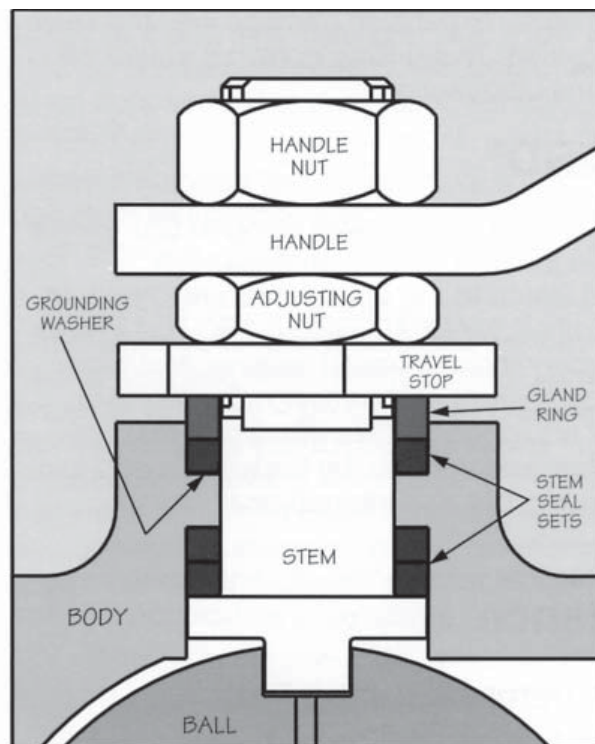
(Sizes 1/2" - 12" Full Port, 2" - 12" Regular Port)
